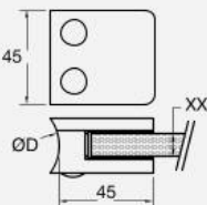
Small Square (45 x 45 mm) for Glass 6 to 10.76 mm
