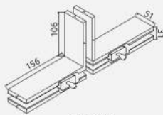
Double Pivot Door Patch for Adjoining Doors
