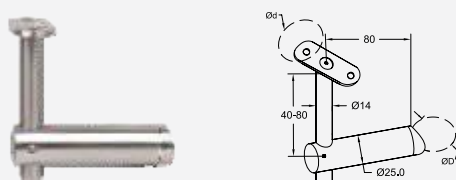
Handrail Bracket for Round Post & Flat Saddle
