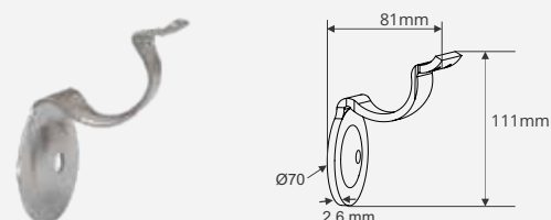
Stainless Steel Wall Bracket
