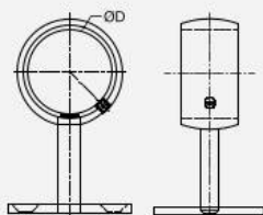
Tube Support with Ring Decorative Through Hole
