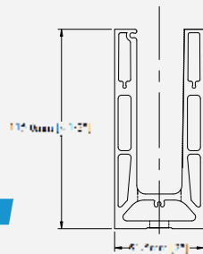
Top Mount Aluminum Channel
