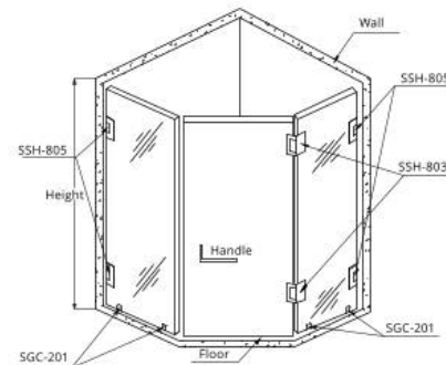
Wall to glass Shower layout
