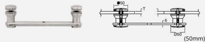
Two Way Glass Holder w/o Post Holder dia 50 mm
