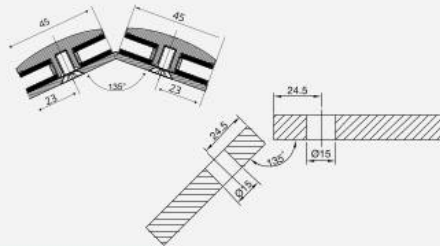
Connector to join Glass to Glass Panel at 135°
