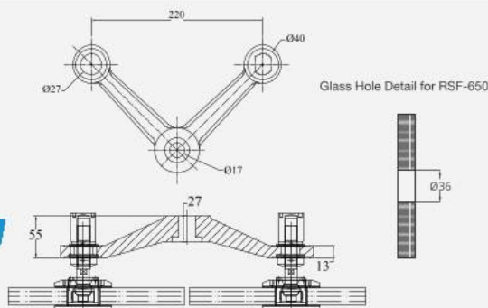
Two Way Spider Fitting at 90° Angle
