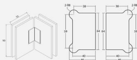
Hinge to join Glass Door with Fixed Glass at 90°
