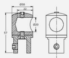
Connector to join Supporting Pipe on end & Glass Panel
