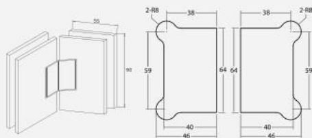
Hinge to join Glass Door with Fixed Glass at 135°
