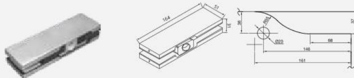
Top Patch for Glass Door
