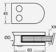
Big D (63 x 45 mm) for Glass 6 to 12.76 mm
