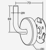
Wall Bracket with Cover and Lock Plate without Saddle
