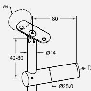
Swivel Handrail Bracket for Flat Post
