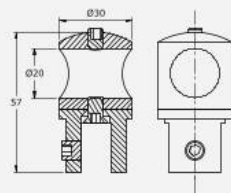
Connector to join Supporting Pipe & Glass Panel
