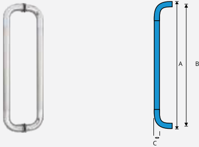
Handle D-Type for Glass Door
