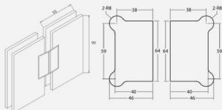
Hinge to join Glass Door with Fixed Glass at 180°
