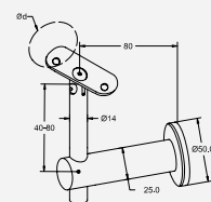
Swivel Handrail Bracket for Wall Mounting
