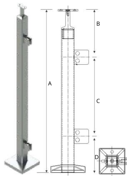
Square End Post with Two Small Glass Clip
