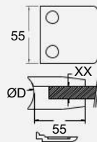
Big Square (55 x 55 mm) with Bottom Plate for Glass 6 to 12.76 mm
