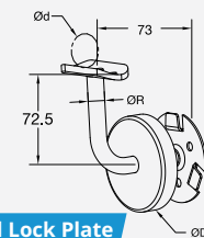
Wall Bracket with Cover and Lock Plate
