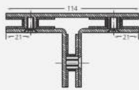
Connector to join Glass to Fin Glass Panel (T-Type)
