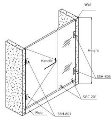
Wall to glass Shower layout
