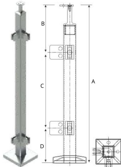
Square Corner Post with Four Small Glass Clip at 90°
