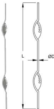
Pickets of Double arc Pattern
