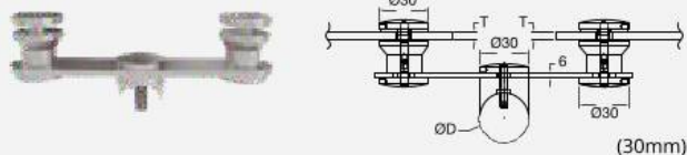
Two Way Glass Holder with Post Holder dia 30 mm
