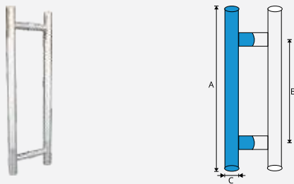
Handle H-Type for Glass Door
